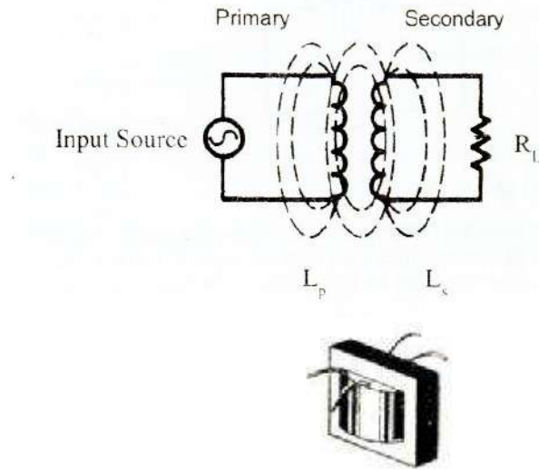
TRANSFORMER
