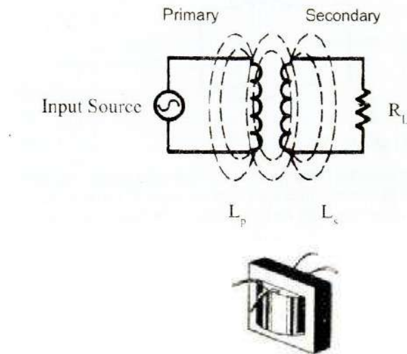
TRANSFORMER
